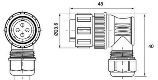
Cable outer diameter range:6-10mm
