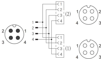
Contact assignment of M12 T1 connector
