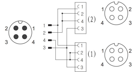
Contact assignment of M12 T2 connector
